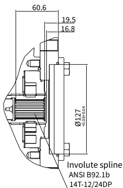
"C6" type through drive
