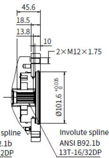
"B1" type through drive
