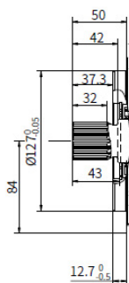
"C5" type spline shaft DIN 5480 W35×2×16×9g
