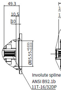
"A2" type through drive
