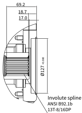
"CF" type through drive
