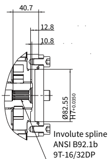
"A1" type through drive
