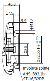
"A1" type through drive
