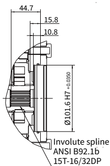
"B3" type through drive
