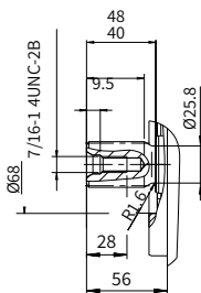
"B4" type spline shaft ANSI B92.1b 1 1/4 in 14T 12/24DP
