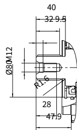
"CA" type spline shaft DIN 5480 W35×2×16×9 g
