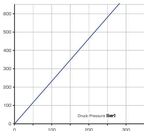
Diagramm Kraftaufwand am Hebel L=430 mm Diagram Pressure-Force; L=430mm
