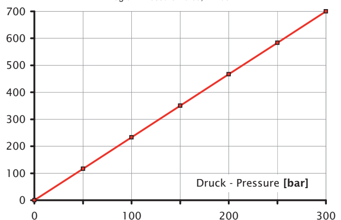
Diagramm Kraftaufwand am Hebel; L=430mm Diagram Pressure-Force; L=430m
