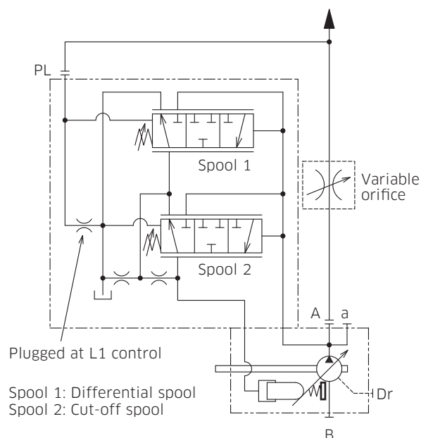
Hydraulic circuit
