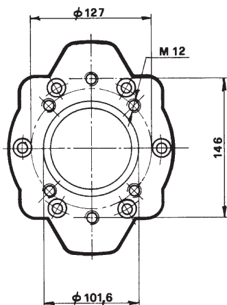
SAE B 2-4 holes 30421 - 30422
