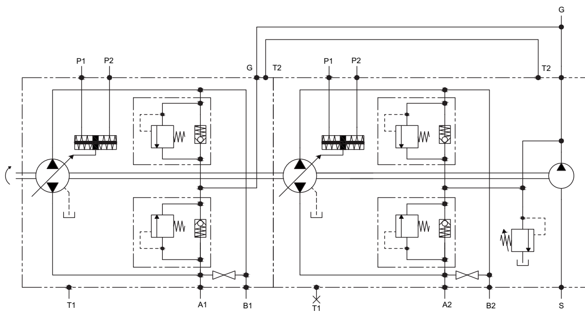
HYDRAULIC DIAGRAM
