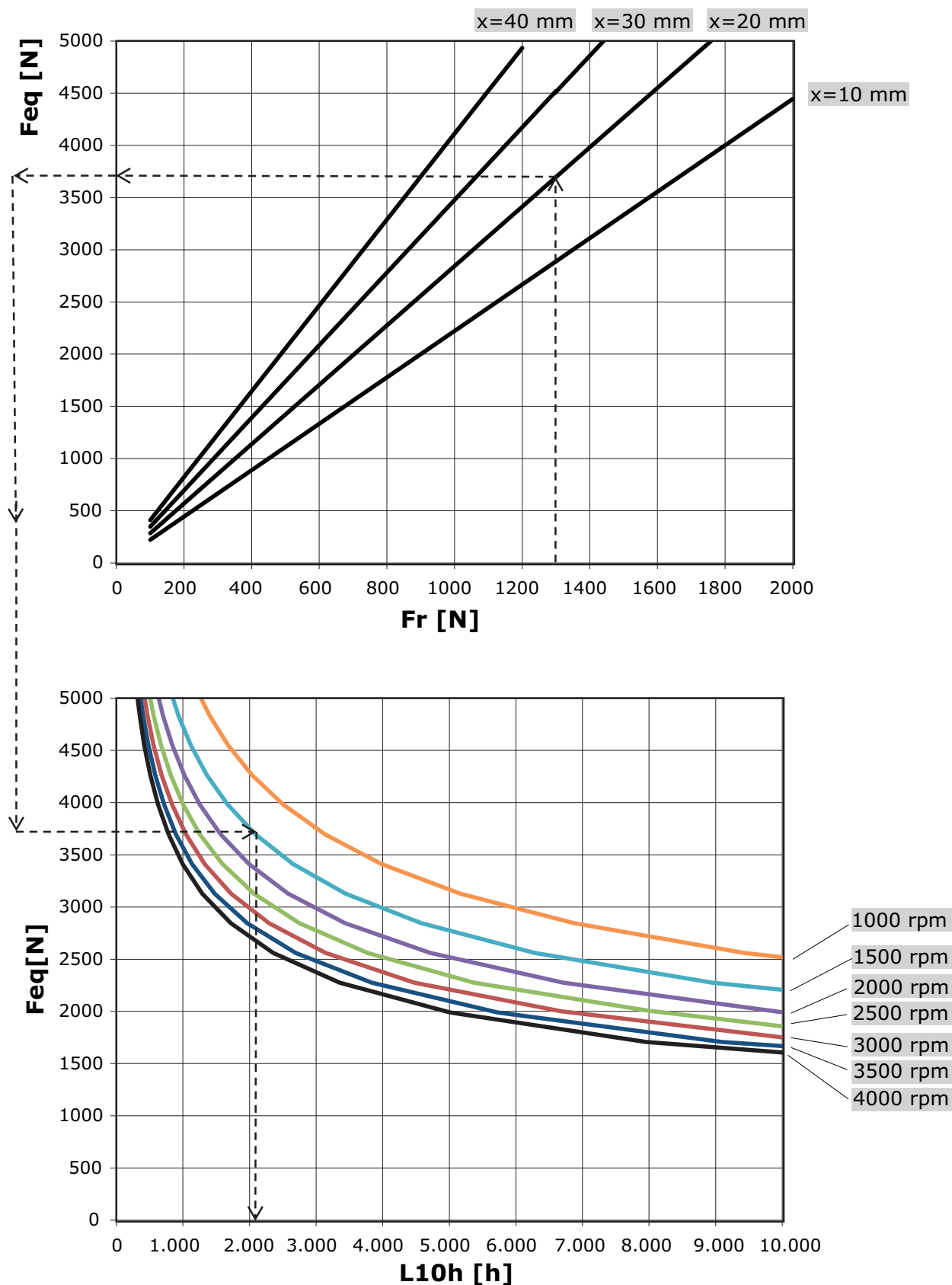
DIAGRAMMA CUSCINETTI • DIAGRAM BEARING EXPECTED LIFE
